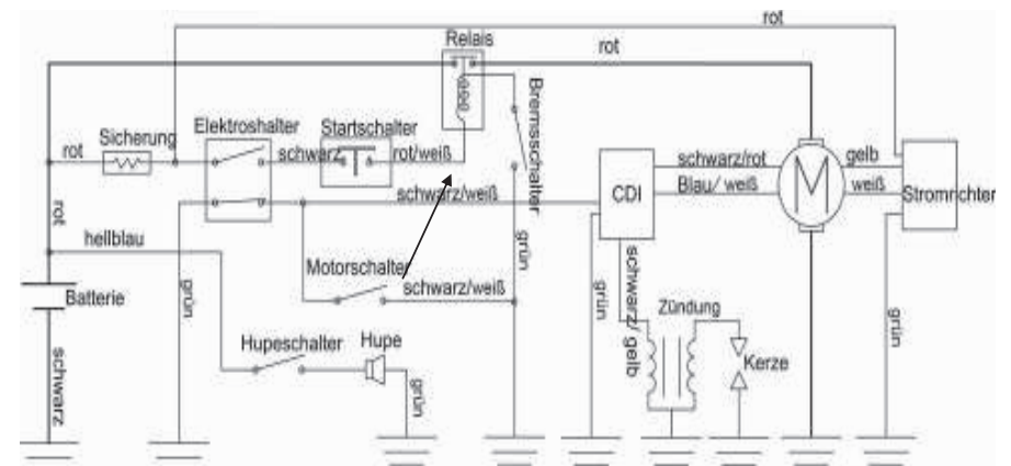
SCHALTPLAN-KXD502C:
